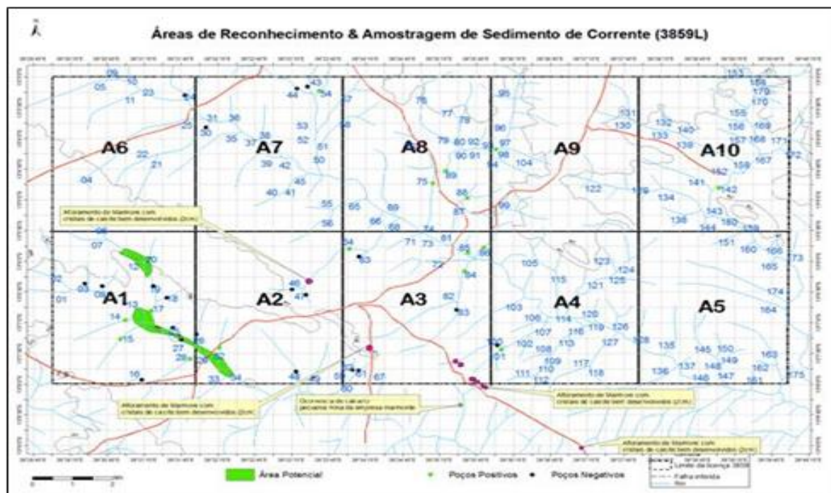
Figure 2 - Sample sediment map (11.000ha). In Block A1 seven shafts have been opened and Ruby samples have been found.
